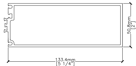
Structural Silicone Glazing
