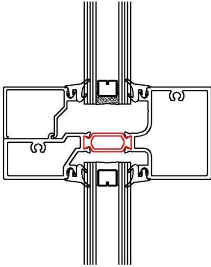
HORIZONTAL MULLION
